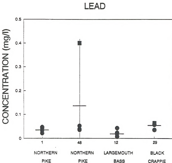
Figure 12. Comparison of replicate analyses from the same fish fillet. Squares represent the value of the initial determination while the circles represent lead from randomly selected tissue samples. Mean concentration (horizontal bar) and 95% confidence intervals are shown for the four samples.
